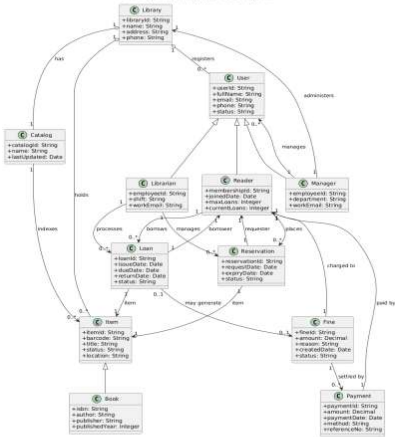
Library Management System - Class Diagram
