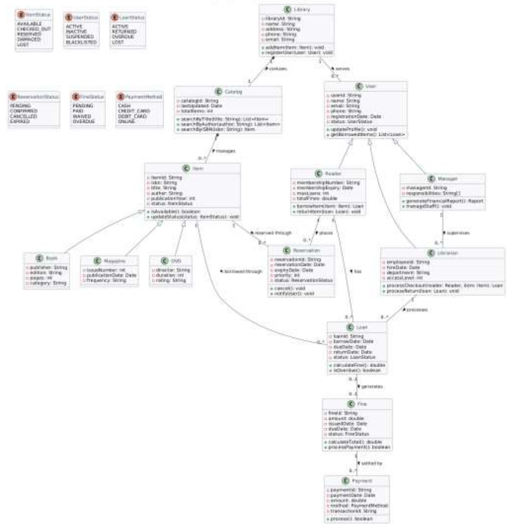
Library Management System - Class Diagram
